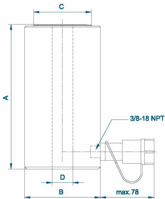
WH-1 Application with the use of 20tn hollow piston cylinder
